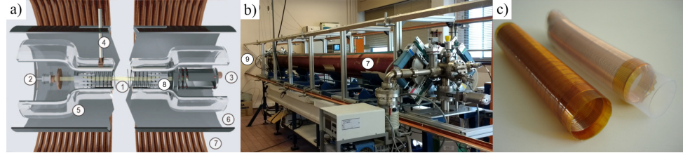
FIG. 1. (Color online) (a) TWT structure (Reproduced from [F. Doveil, A. Macor, and Y. Elskens, "Direct observation of a 'devil's staircase' in wave-particle interaction", Chaos 16, 033103 (2006)], with the permission of AIP Publishing): (1) helix; (2) electron gun; (3) trochoidal velocity analyzer; (4) movable antenna; (5) glass vacuum tube; (6) slotted rf ground cylinder; (7) main magnetic coil; (8) resistive rf termination to reduce reflections. (b) Picture of the TWT showing its magnetic coils: (7) main coil producing the magnetic field B_z to confine the beam, and (9) rectangular coils generating B_x and B_y for beam tilt correction. (c) Helix wrapped in a dielectric polyimide tape.
