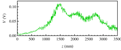
FIG. 11. Wave amplitude (30 MHz) after interaction with an electron beam ( I_b = 326 \mu\text{A} ) emitted with higher velocity than the wave phase velocity.
