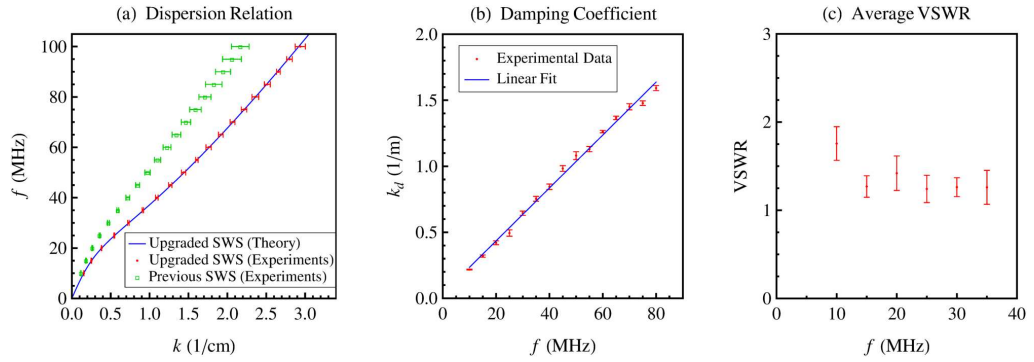
FIG. 6. (Color online) (a) Theoretical dispersion relation (blue solid curve) and experimental data (full red circles) for the upgraded SWS, and experimental points (green open squares) for the previous SWS. (b) Damping coefficient and (c) average voltage standing wave ratio (VSWR) as a function of wave frequency for the upgraded SWS.
